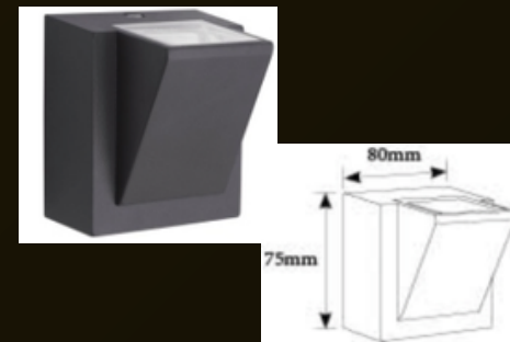
NE SINGLE SIDE K TYPE 3W
