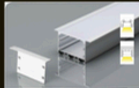
DIMENSION 60X60X35 MM PCB SIZE 45 MM
