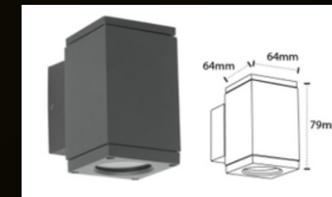
NE SQ CYLINDER SINGLE SIDE 6W
