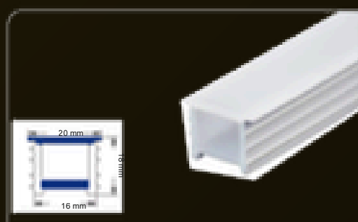
FLEX NEON 1616 CONCEALED
